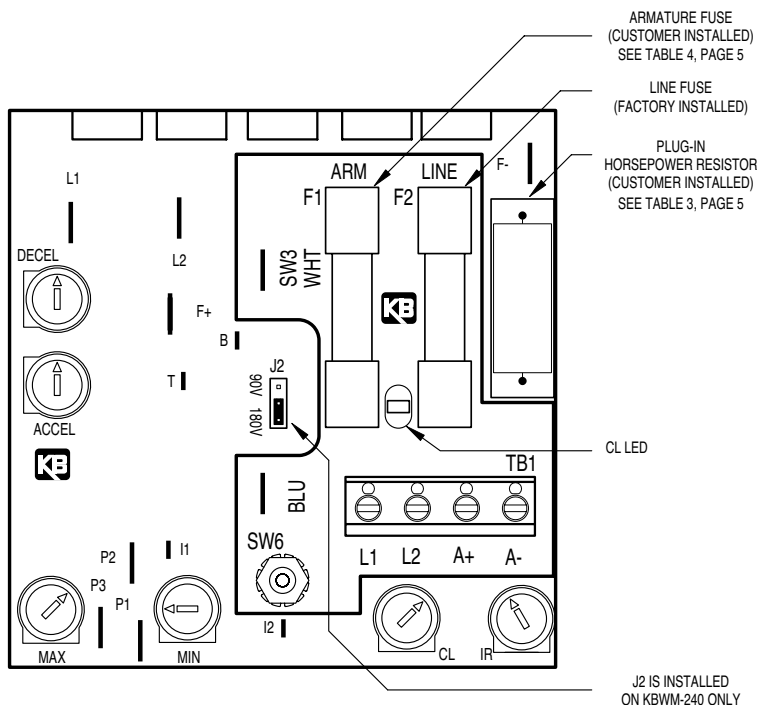
FIGURE 1 – CONTROL LAYOUT
